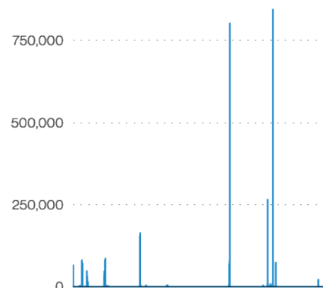
Figure 12. Time between SIEM events (n=1,335,343)
