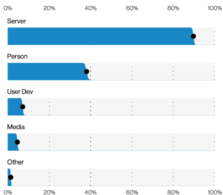
Figure 29. Top Assets in breaches (n=4,717)
