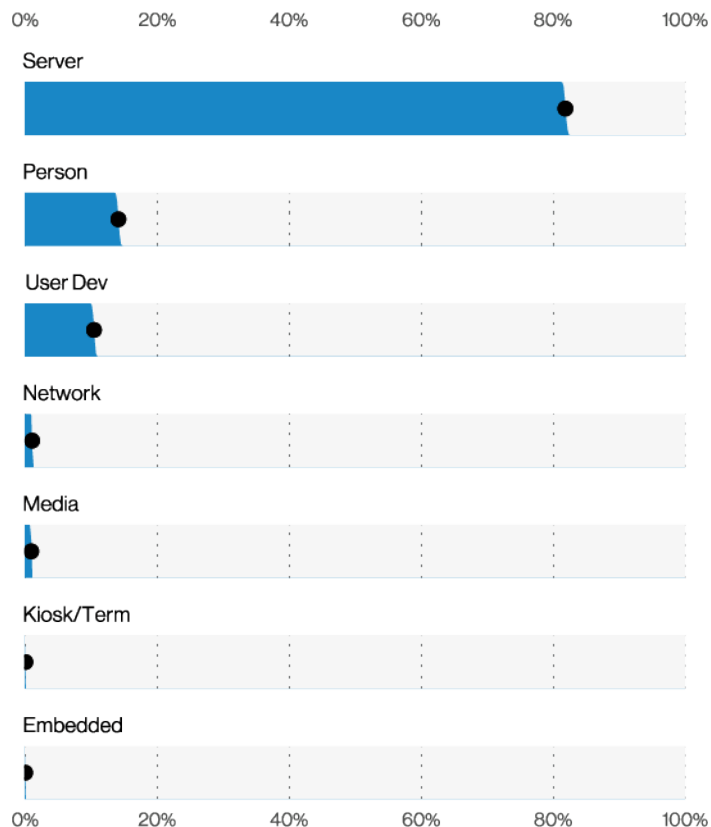
Figure 27. Assets in incidents (n=27,634)
