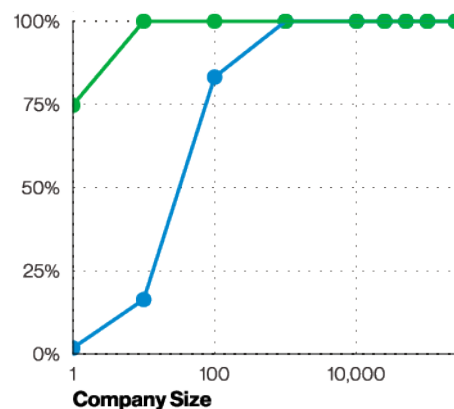
Figure 34. Probability that someone in the company will receive a malicious URL or install a malicious APK based on organization size (n=5,440,000)
